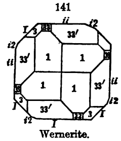
Wernerite.
